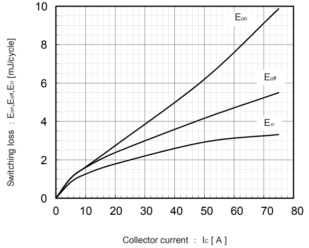
Switching Loss vs. Collector Current (typ.) V_{DC}=600V, V_{CC}=15V, T_j=25^\circ C
