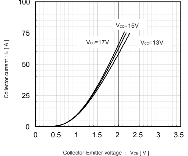
Collector current vs. Collector-Emmitter voltage T_j=125^\circ\text{C} [Terminal] (typ.)
