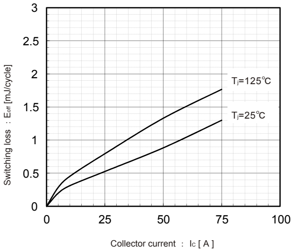
Switching Loss vs. Collector Current (typ.) V_{bc}=300V, V_{cc}=15V
