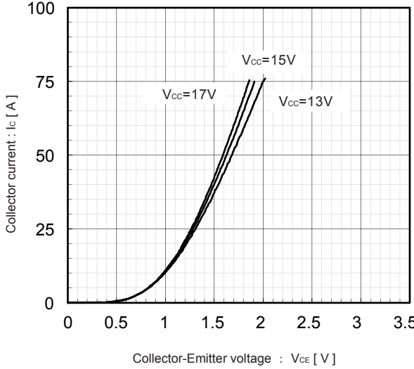
Collector current vs. Collector-Emmitter voltage T_j=125^\circ\text{C} [Chip] (typ.)
