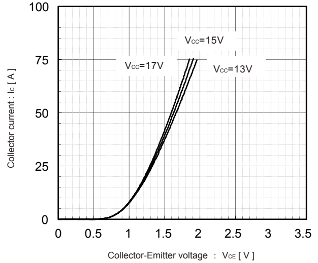
Collector current vs. Collector-Emmitter voltage T_j=25^\circ\text{C} [Terminal] (typ.)
