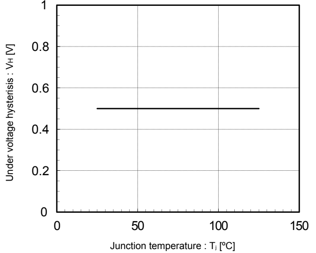
Under voltage hysteresis vs. Junction temperature (typ.)
