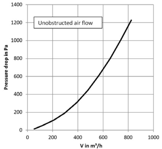
Fig. 10: Pressure drop \Delta p versus flow rate V
