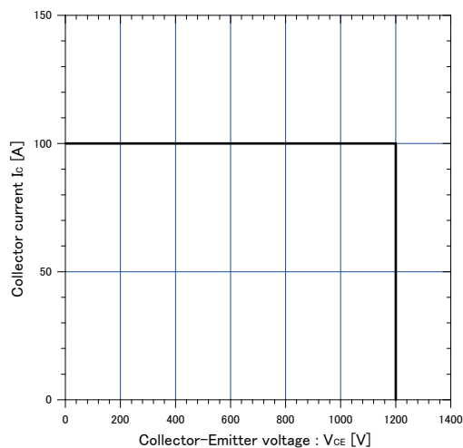
Graph.13 Reverse biased Safe Operating Area T_{\leq 175^{\circ}\text{C}}, V_{\text{GE}} = +15\text{V}/0\text{V}, R_{\text{G}} = 10\Omega
