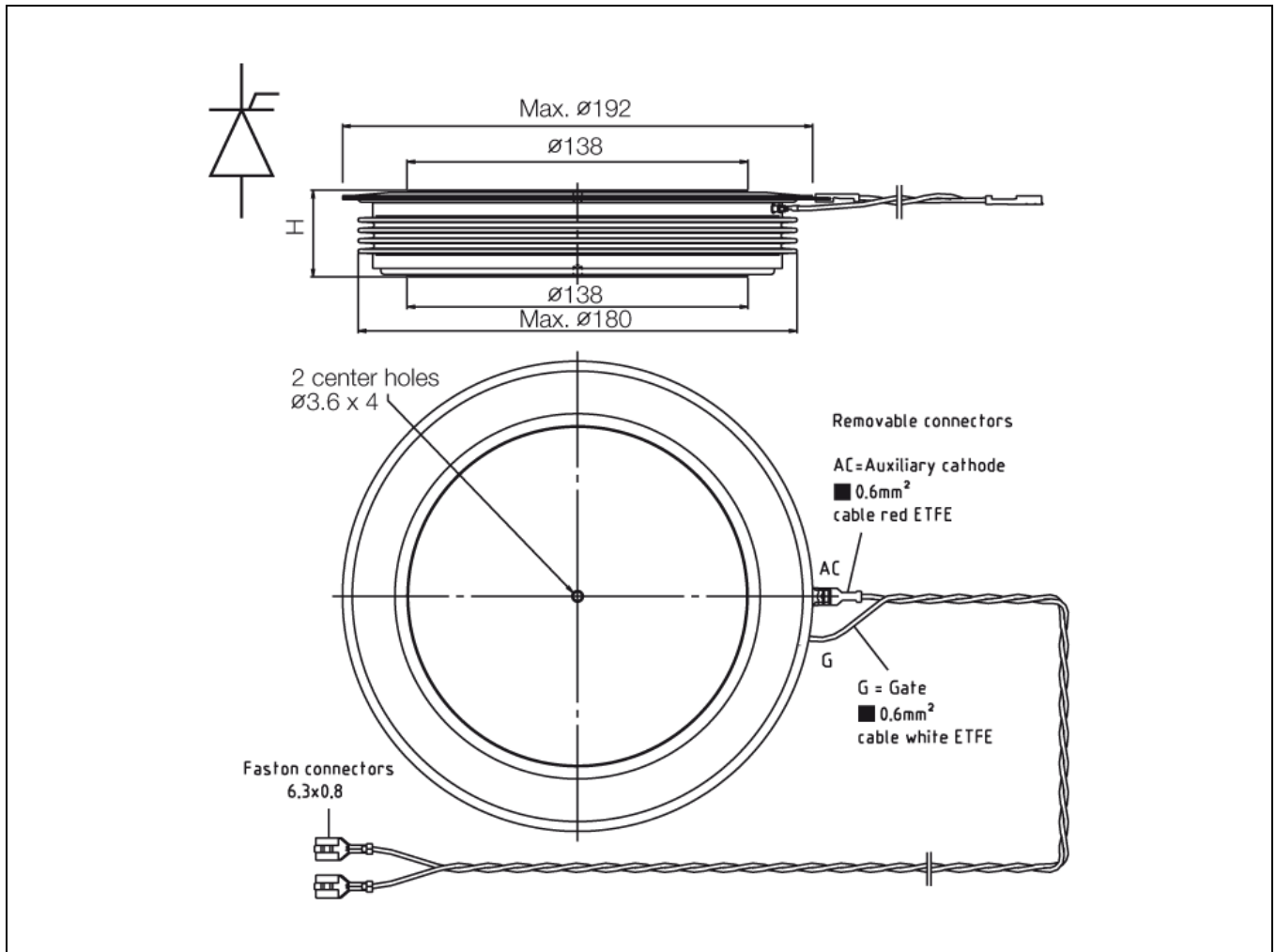
Fig. 13 Device Outline Drawing
