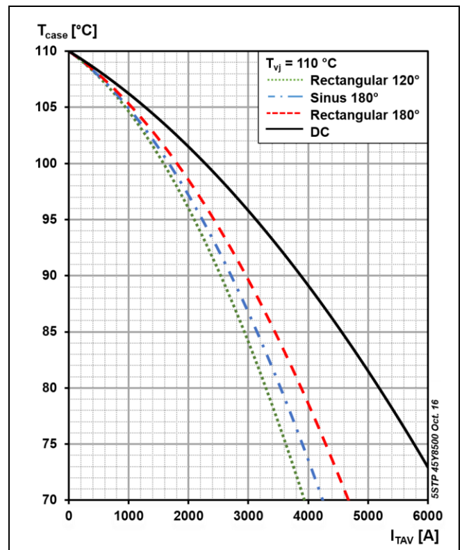
Fig. 4 Max. permissible case temperature vs. mean on-state current, switching losses ignored
