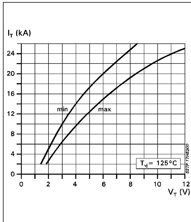
Fig. 3 On-state voltage characteristics, T_{vj} = 125\text{ }^\circ\text{C} , 10 ms half sine
